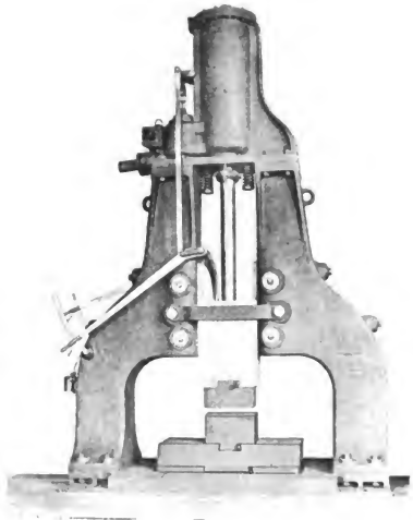
Fig. 4946. Double Frame Steam Hammer. Niles-Bement-Pond Co.
